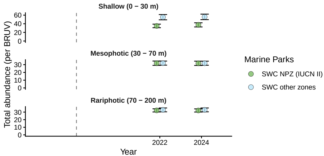
Figure 10.1: Demersal fish - Total abundance: benchmark plots by zone and depth contour from stereo-BRUV groundtruthing. SWC = South-west Corner Marine Park (Commonwealth).
